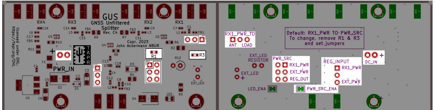
Figure 5: Gus Power Configuration Top (left) and Bottom (right)
