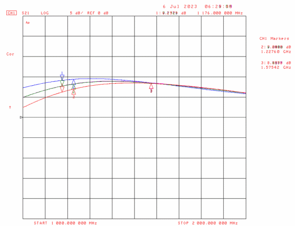
Figure 2: Gain of All Four Ports
