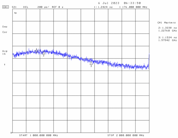
Figure 3: RX Port 1 Group Delay
