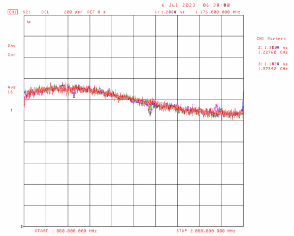
Figure 4: Group Delay of All Four Ports
