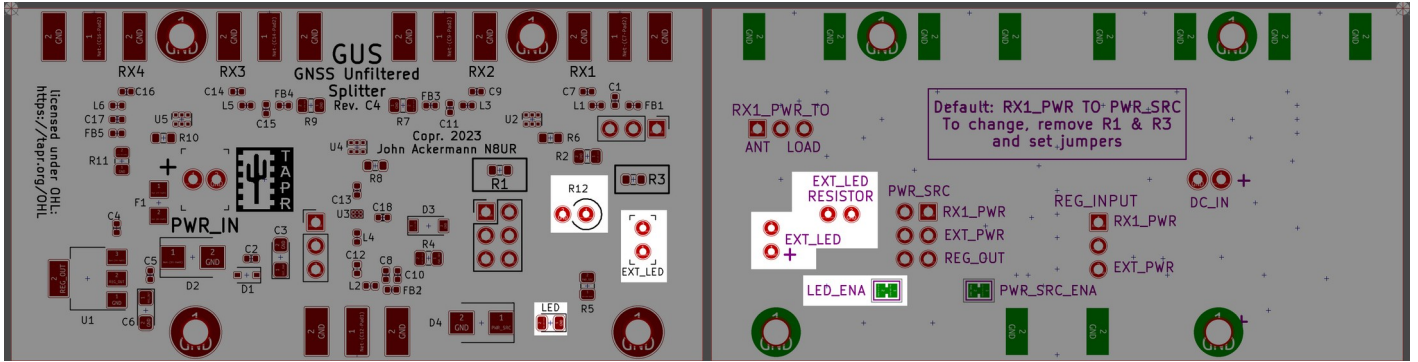
Figure 6:Gus LED Configuration Top (left) and Bottom (right)
