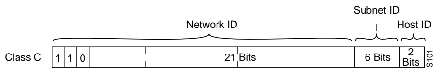
Figure 2-2 Class C Subnet Address Format
