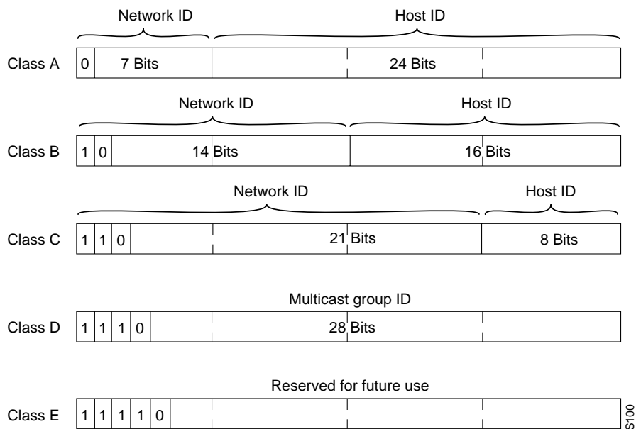
Figure 2-1 IP Address Formats
